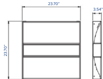
Model LGL-STFR-22
