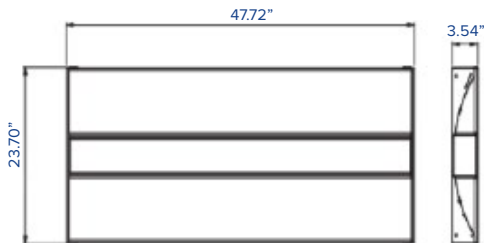
Model LGL-STFR-24
