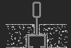
9/16" Slot Ceiling
