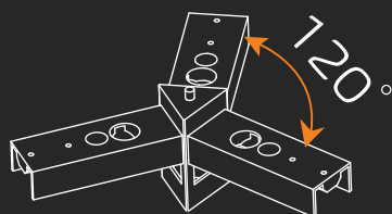
"Y" Connector
